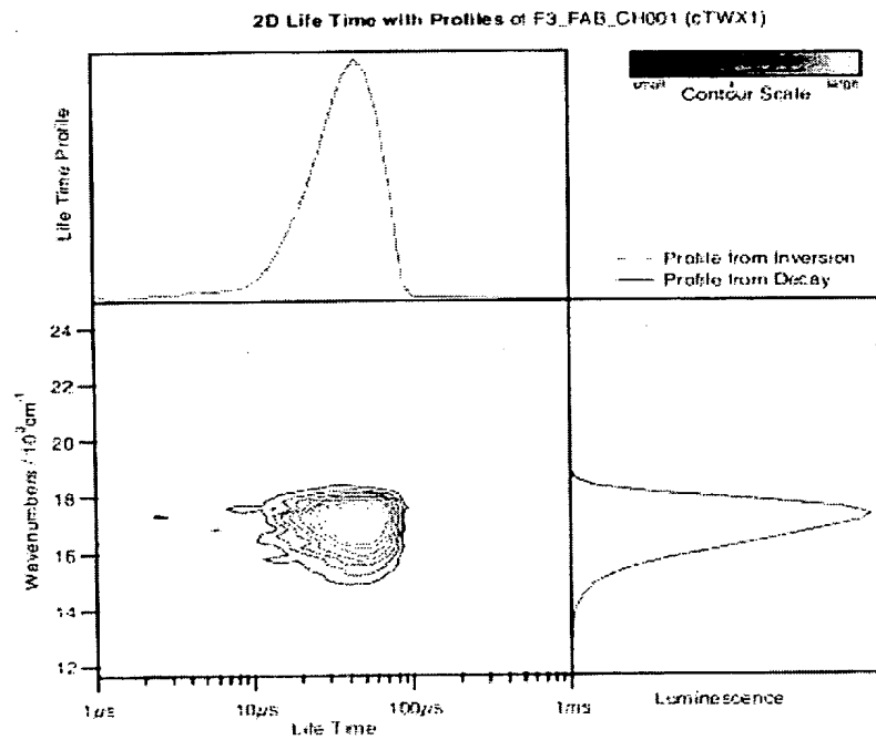
FIGURE 4 (I)/FAB Ratio 1:1 in Cyclohexane at 80K
